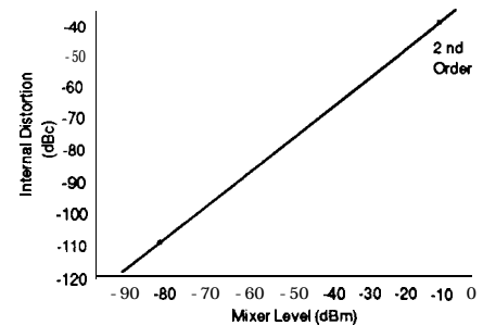
Fig. 66. Extended second-order distortion graph.
