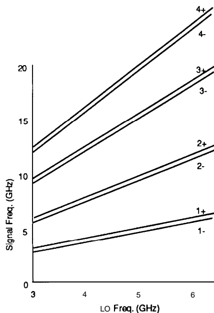
Fig. 61. Tuning curves for n = 1 through 4 in the high-band, low-IF case.
