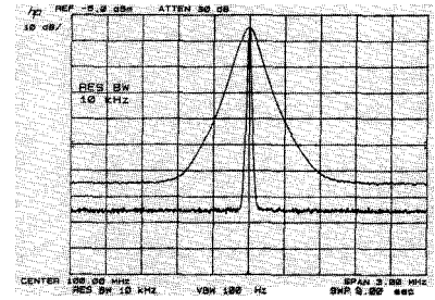
Fig. 43. Displayed noise level changes as 10*\log(BW_o/BW_i) .
