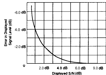
Fig. 56. Error in displayed signal amplitude due to noise.
