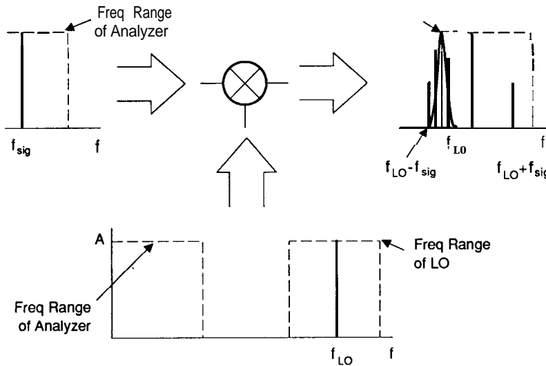
Fig. 9. The LO must be tuned to f_{IF} + f_{sig} to produce a response on the display.
