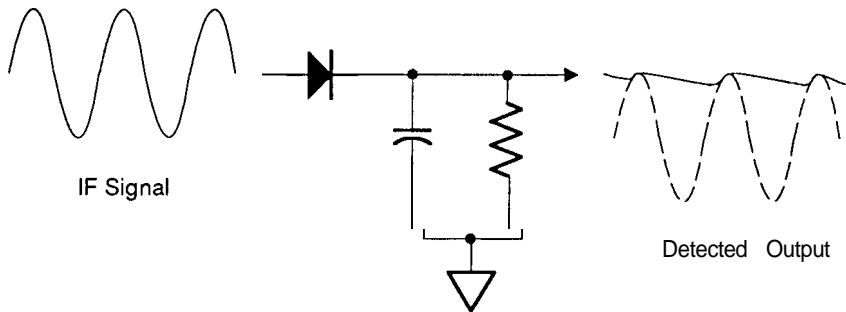
Fig. 22. Envelope detector.
