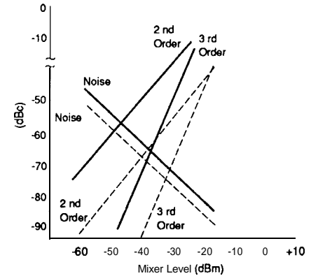
Fig. 55. Dynamic range for 1.5-dB maximum error.
