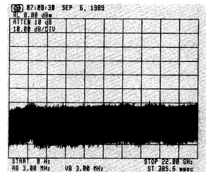
Fig. 72. Fundamental mixing across the entire tuning range gives the HP 71210 the same sensitivity at 22 GHz as at 1 GHz.
