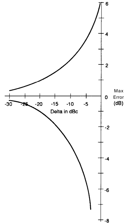
Fig. 54. Uncertainty versus difference in amplitude between two sinusoids at the same frequency.
