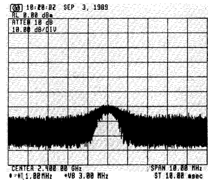
Fig. 24. Spectrum analyzers display signal plus noise.
