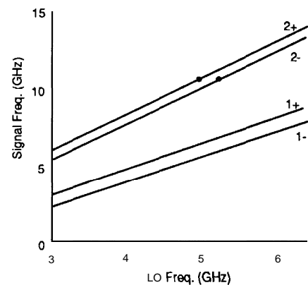
Fig. 66. A response at a given LO frequency does not uniquely determine signal frequency.
