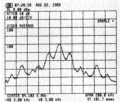
Fig. 29. Video (analog) filtering and video (digital) averaging yield different results on an FM broadcast signal.
