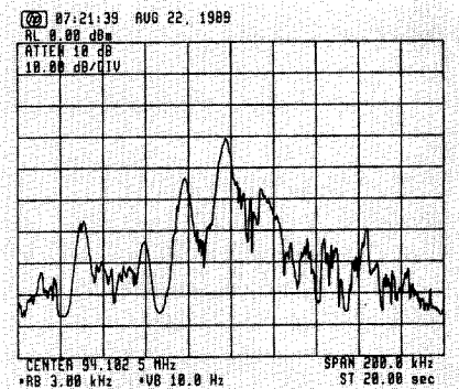
Fig. 29A. Analog filtering.
