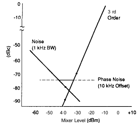
Fig. 53. Phase noise can limit third-order intermodulation tests.
