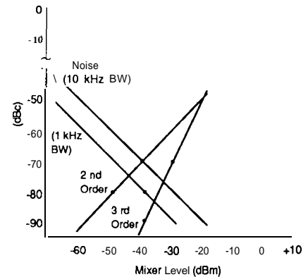
Fig. 52. Reducing resolution bandwidth improves dynamic range.
