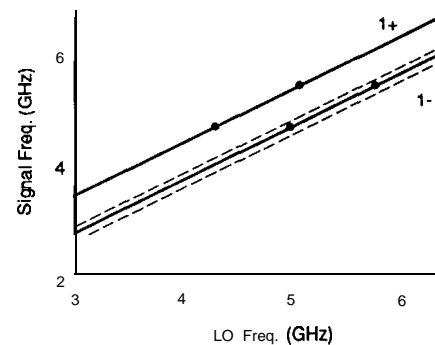
Fig. 66. A preselector allows a signal to reach the mixer only when the analyzer is tuned to receive the signal.
