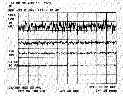
Fig. 28. Effect of video (digital) averaging for 1, 5, 20, and 100 sweeps (top to bottom).
