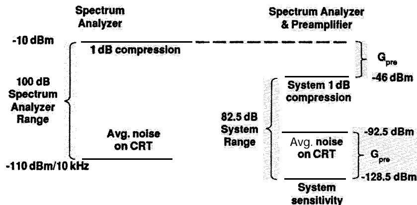
Fig. 45. If the displayed noise goes up when a preamplifier is connected, measurement range is diminished by the amount the noise changes.
