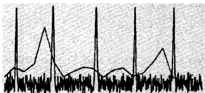
Fig. 34. The actual comb and results of the sample display mode over a 500-MHz span. When resolution bandwidth is narrower than the sample interval, the sample mode can give erroneous results. (The sample trace has only 20 points to exaggerate the effect.)
