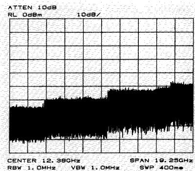
Fig. 63. Steps in the noise floor indicate changes in sensitivity with changes in LO harmonic used in the mixing process.
