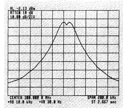
Fig. 12. Two equal-amplitude sinusoids separated by the 3 dB BW of the selected IF filter can be resolved.
