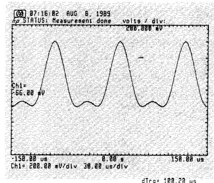
Fig.1. Complex time-domain signal.
