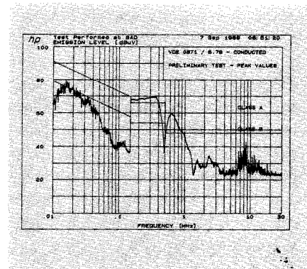
Fig. 6. Conducted emissions plotted against VDE limits as part of EMI test.
