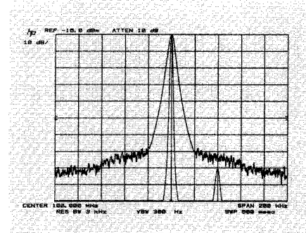
Fig. 20. Phase noise can prevent resolution of unequal signals.
