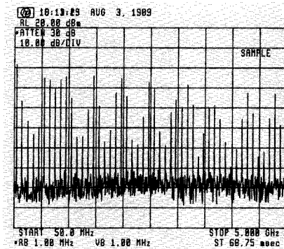
Fig. 33. A 5-GHz span of a 100-MHz comb in the sample display mode. The actual comb values are relatively constant over this range.
