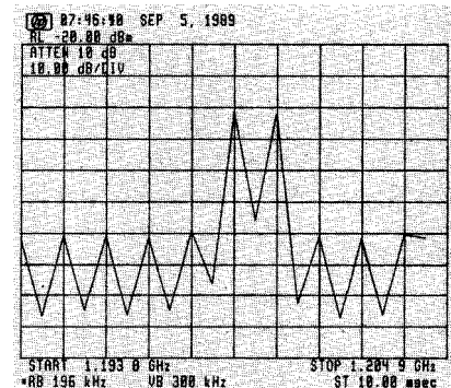
Fig. 39. Rosenfell when signal peak falls between data points (fewer trace points exaggerate the effect).
