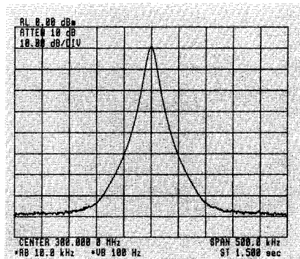
Fig. 8. Typical spectrum analyzer display with control settings.
