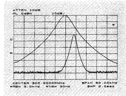
Fig. 13. A low-level signal can be lost under skirt of the response to a larger signal.
