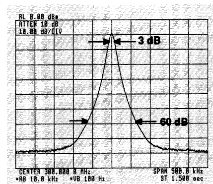
Fig. 14. Bandwidth selectivity, ratio of 60 dB to 3 dB bandwidths, helps determine resolving power for unequal sinusoids.
