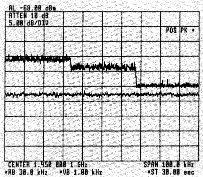
Fig. 27. On analyzers using pos peak display mode, reducing the video bandwidth lowers the peak noise but not the average noise. Lower trace shows average noise.
