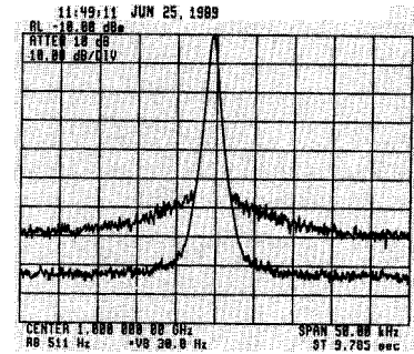
Fig. 64. Difference in phase noise between fundamental and fourth-harmonic mixing.
