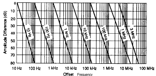
Fig. 16. Resolution versus offset for HP 8566B.
